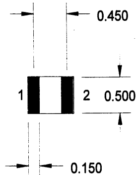
P.C. BOARD PATTERN
