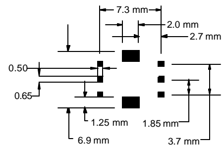
Land Pattern
